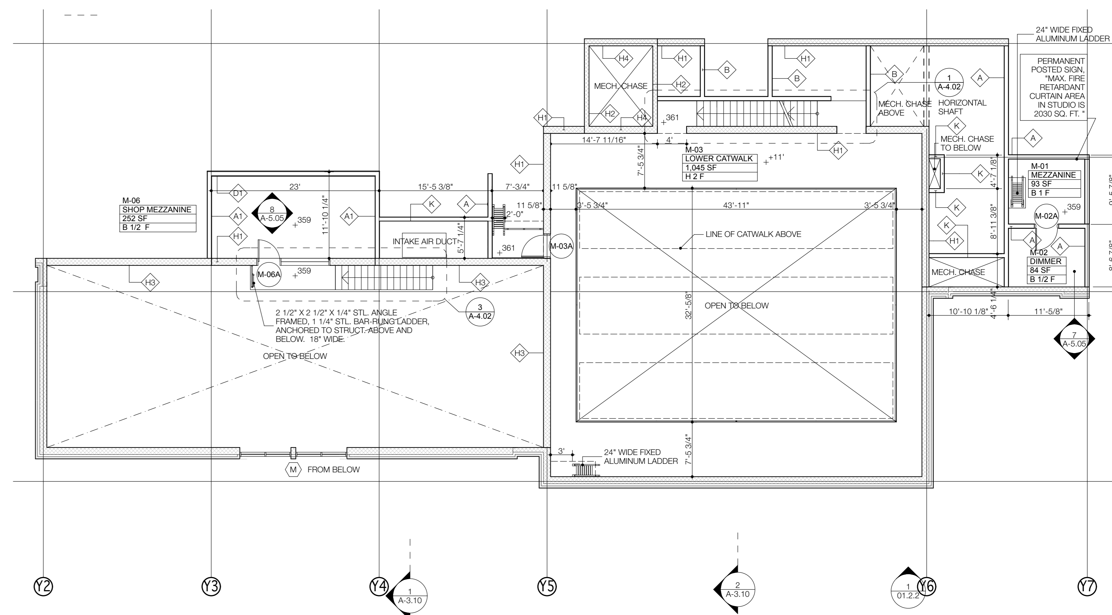
1 A-2.04 LOWER CATWALK PLAN 1/8" = 1'-0" 1/8 INCH EQUALS 1 FT
