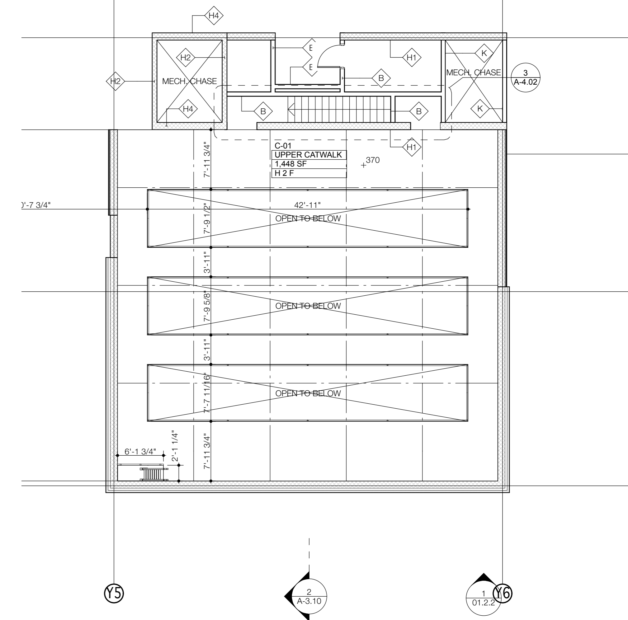
2 A-2.04 UPPER CATWALK PLAN 1/8" = 1'-0"
